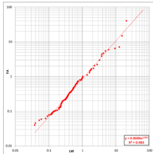
Figure 12-2. QQ plot for LeachWELL vs. FA.
