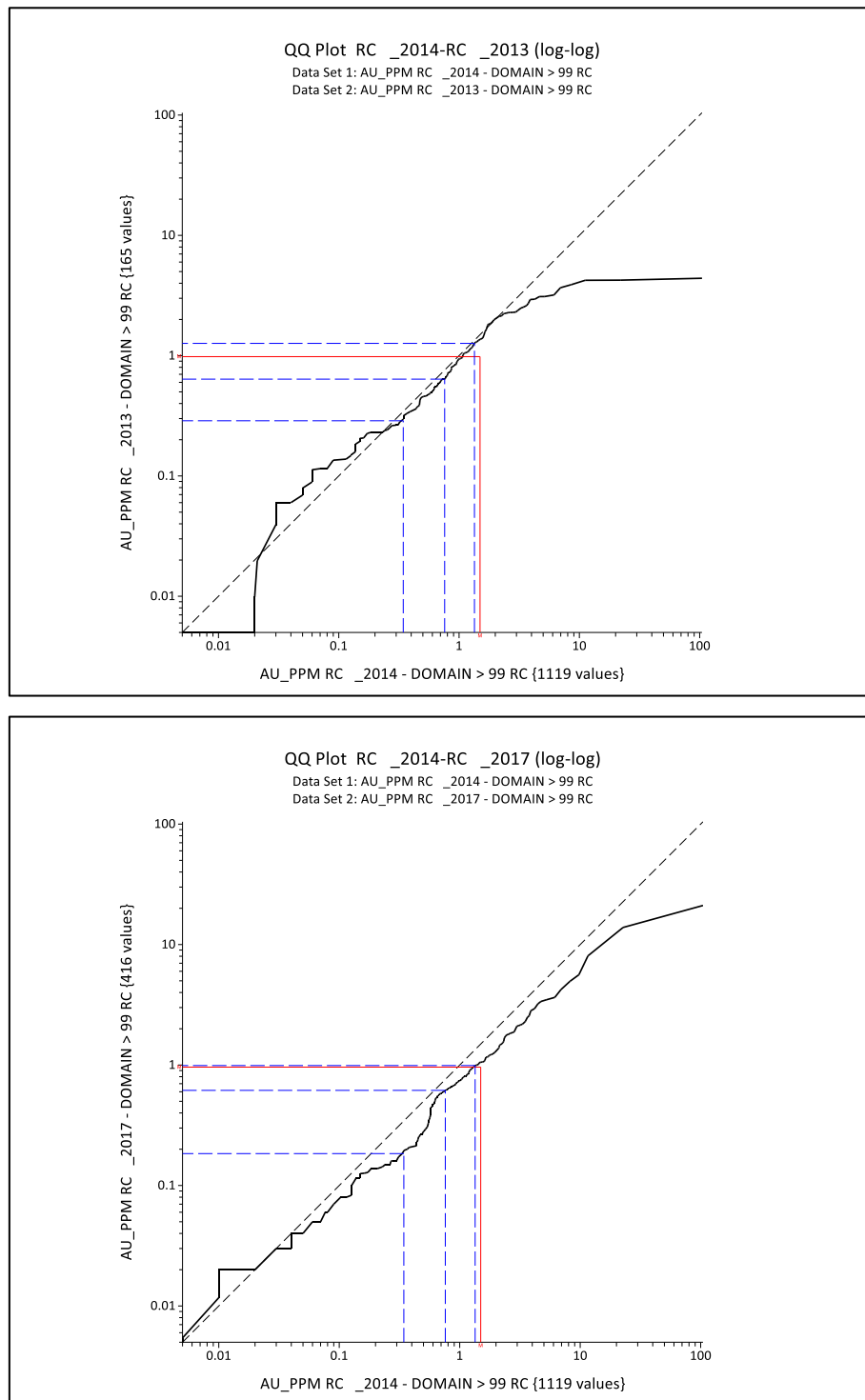
Figure 10-5. QQ plots comparing grades of the 2013 vs. 2014 and 2017 vs. 2014 RC drilling programmes.
