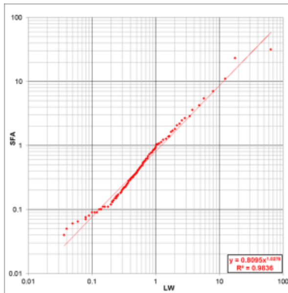
Figure 12-1. QQ plot for LeachWELL vs. SFA.
