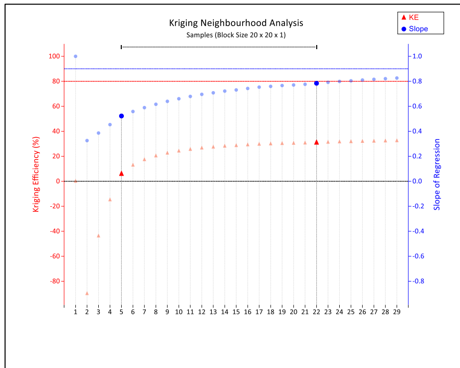
Figure 14-9. KNA plot for optimising number of informing samples.
