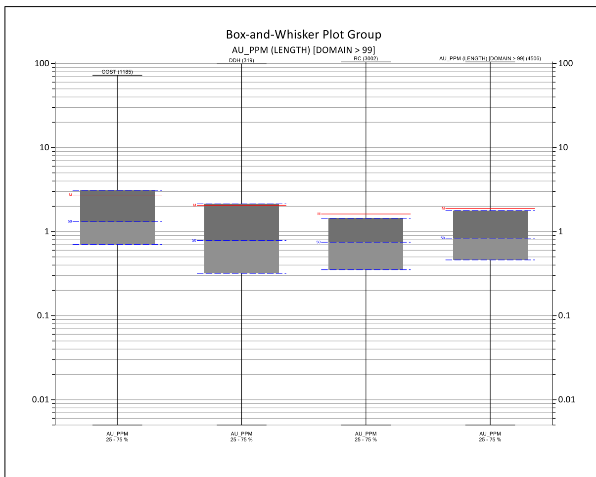
Figure 11-5. Box and whisker plot comparing gold grade by sample type.
